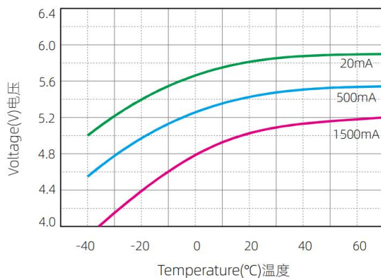
Voltage vs Temperature 电压vs温度
