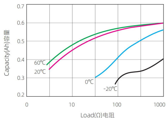
Capacity vs Resistance 容量vs电阻
