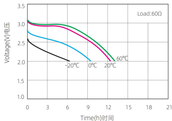
Temperature Characteristics 温度特性
