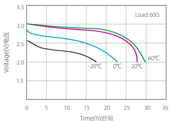
Temperature Characteristics 温度特性
