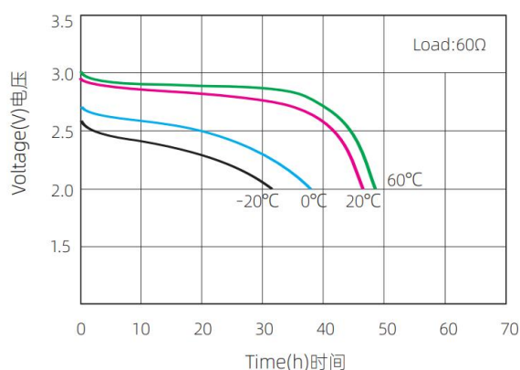
Temperature Characteristics 温度特性
